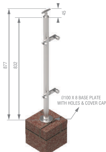
Top Mounted Round Baluster with Double Glass Bracket
