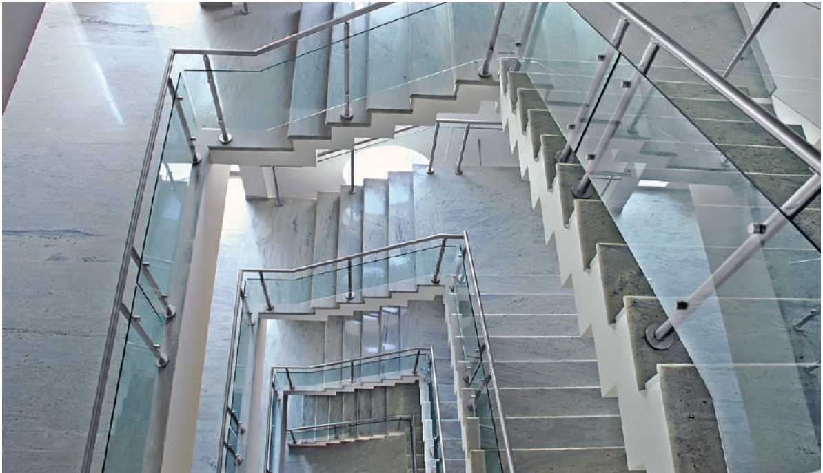
Top Mounted Round Baluster System with Glass - Ø42.4mm (DT15-1-GLS) & Ø50mm (DT12-1-GLS)
