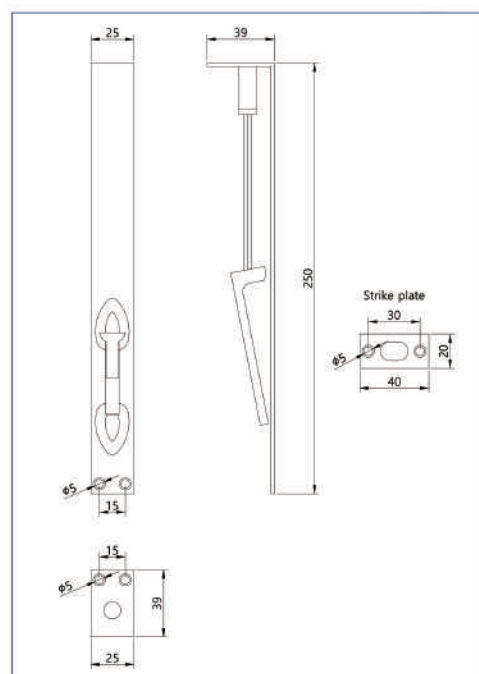
Lever action flush bolts for wooden door 98307012 250mm
