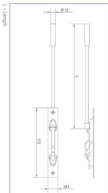
Lever action flush bolts for steel door 98307009 300mm 98487006 600mm
