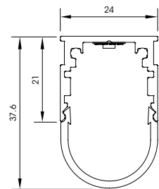
Round cover PMMA diffuse
