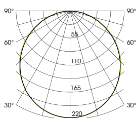
Flat cover PMMA diffuse [F]
